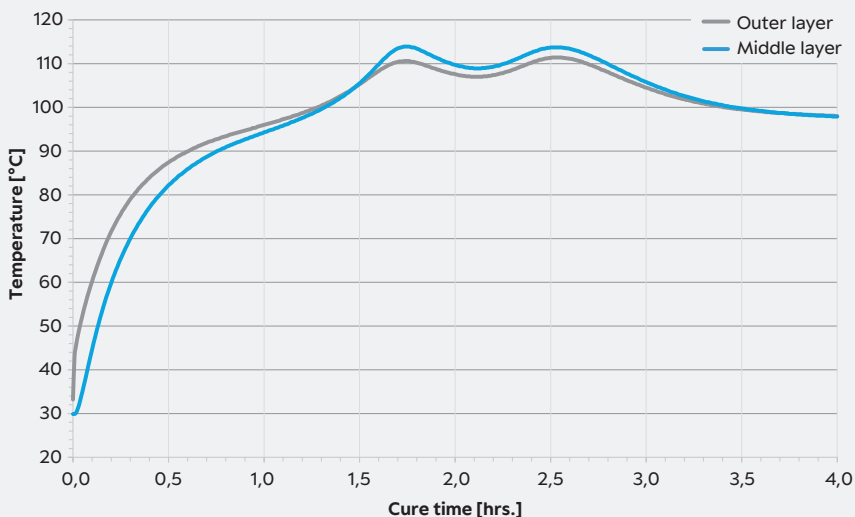
TEMPERATURE PROFILE IN 20 MM LAMINATE CURED AT 95 °C
