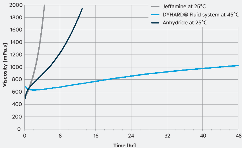
VISCOSITY VERSUS TIME COMPARISON: DYHARD® FLUID SYSTEM AT 45°C VERSUS COMPETITIVE ANHYDRIDE AND JEFFAMINE SYSTEMS AT 25°C
